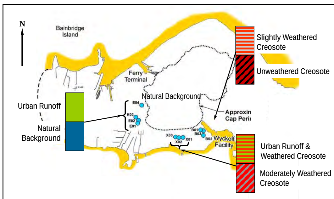
Creosote, urban runoff, and natural background distributions in Eagle Harbor sediment cores (adapted from Brenner et al. , 2001). The vertical columns represent the tops and bottoms of vertically profiled sediment cores (~40 to ~70 cm deep).
