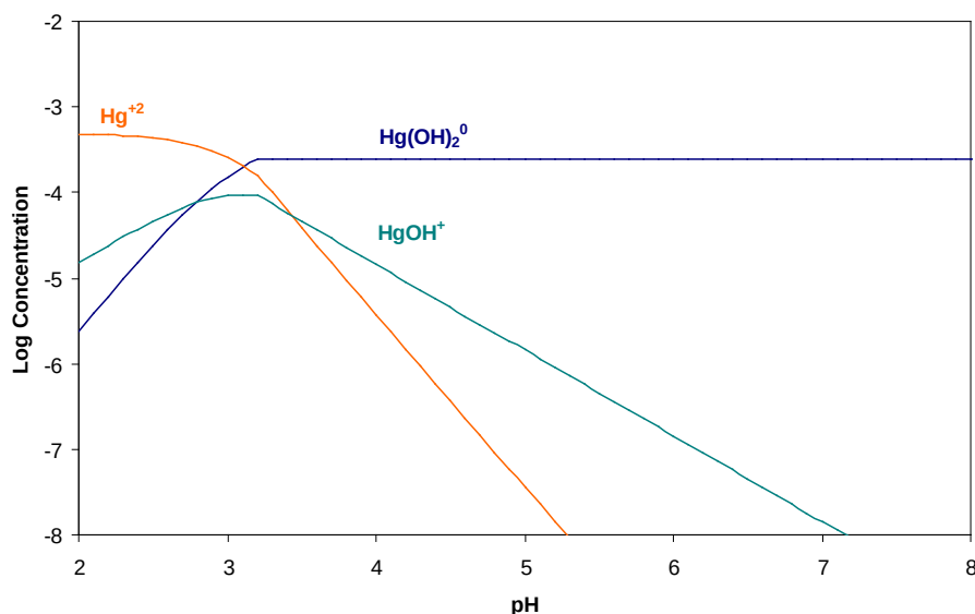
Figure 4-4. Mercury Speciation Plot, \text{Hg}_{\text{tot}} = 10^{-3} \text{ M} (Mercury speciation was modeled using MINTEQ ver. 2.53.)
