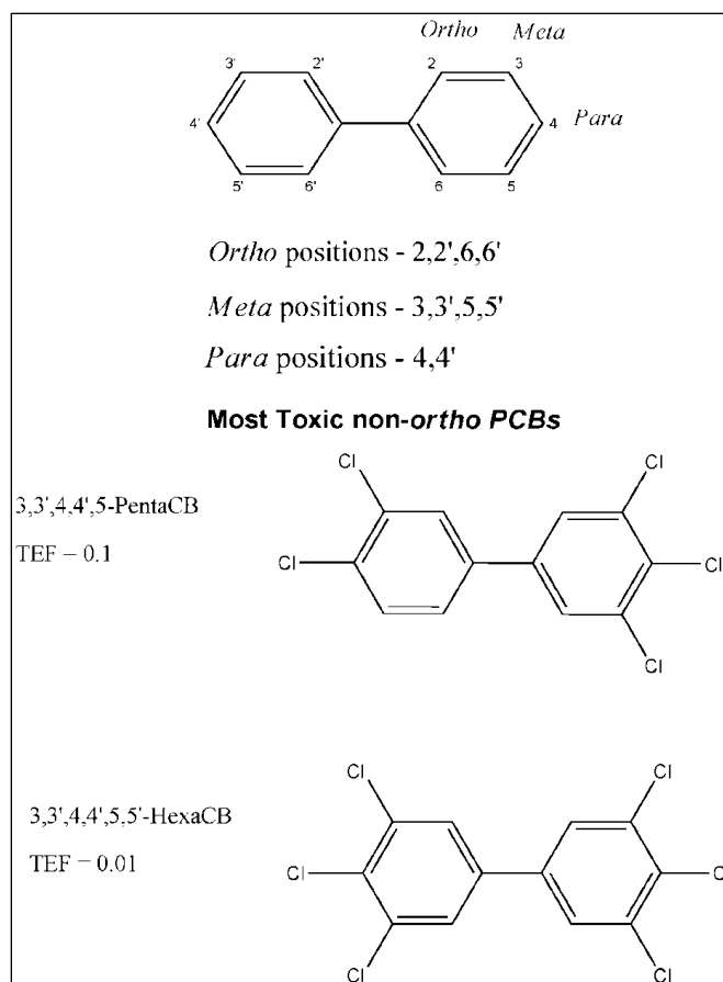
Figure 3-4. Positions of Ortho , Meta , and Para Carbons in PCBs (Structures of the two most toxic non- ortho PCBs are shown based on their TEFs, relative to the toxicity of 2,3,7,8-tetrachloro dibenzo- p -dioxin [Table 3-4].)
